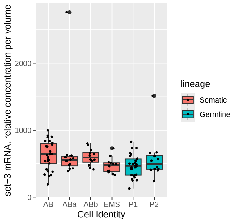
set-3 mRNA, relative concentration
